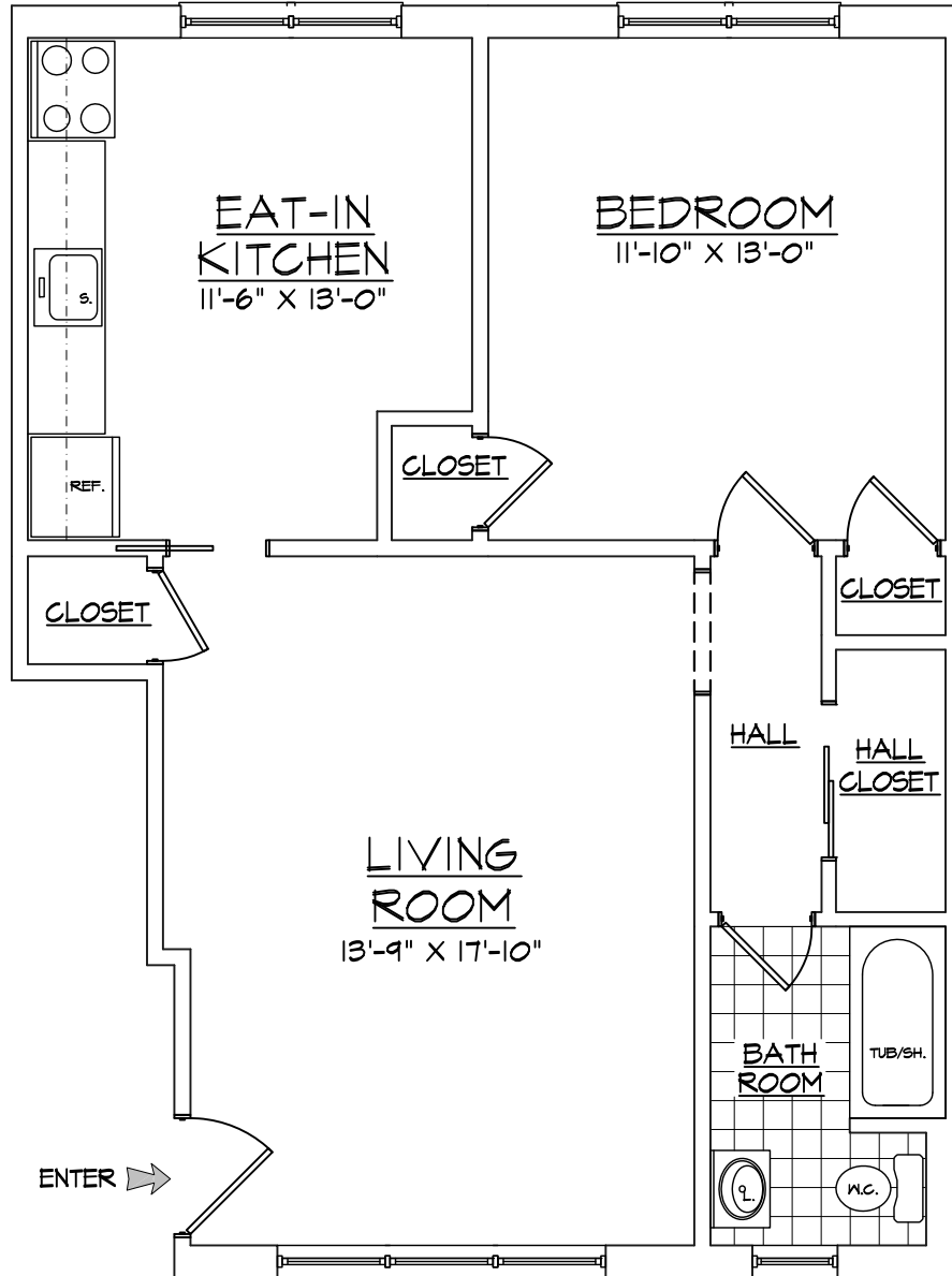
-FIRST FLOOR- ONE BEDROOM w/ E.I. KIT. FLOOR PLAN 707 Sq. Ft. (room sizes are approximate)
