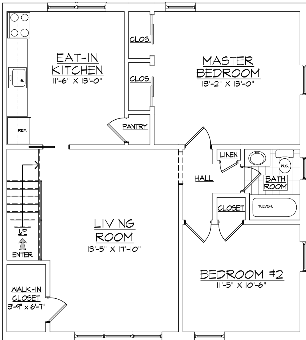
-SECOND FLOOR- TWO BEDROOM w/ E.I. KIT. FLOOR PLAN 904 Sq. Ft.
